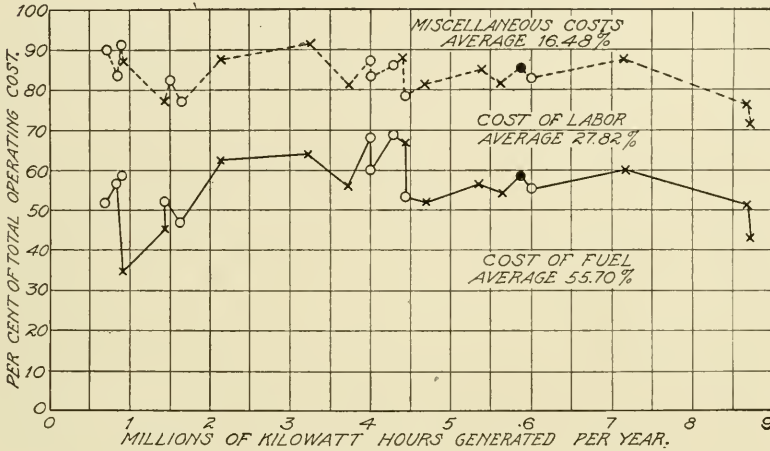
Fig. 162. Curve Showing Per Cent of Total Cost of Fuel, Labor, and Sundries for Given Quantity of Energy Generated Per Year
